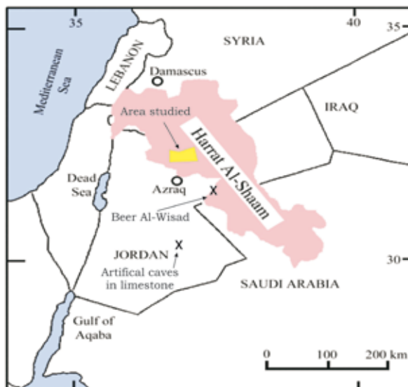
Figure 1. Study area and extent of Hattat Al-Shaam (altered after AL-MALABEH, 1994).
