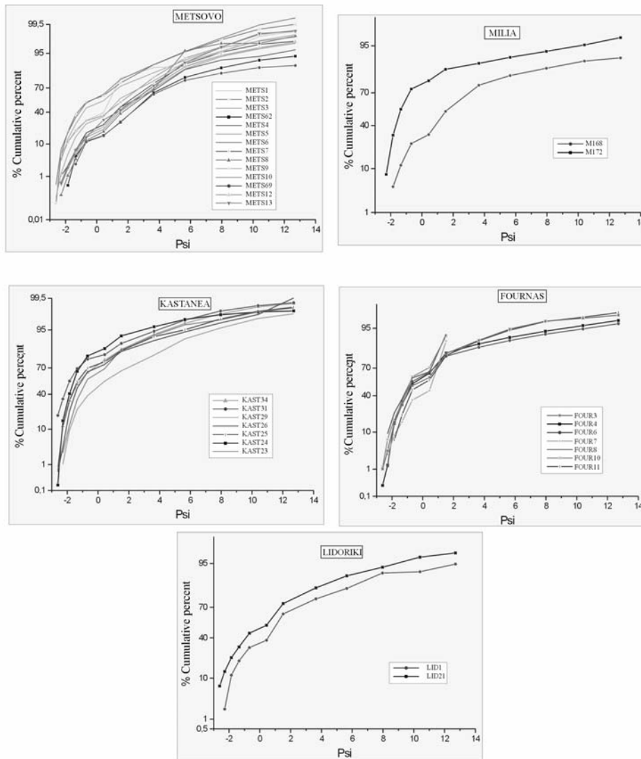
Figure 4. Cumulative curves of settling-velocity ( \text{Psi} ) distributions of samples from the studied cross-sections.
