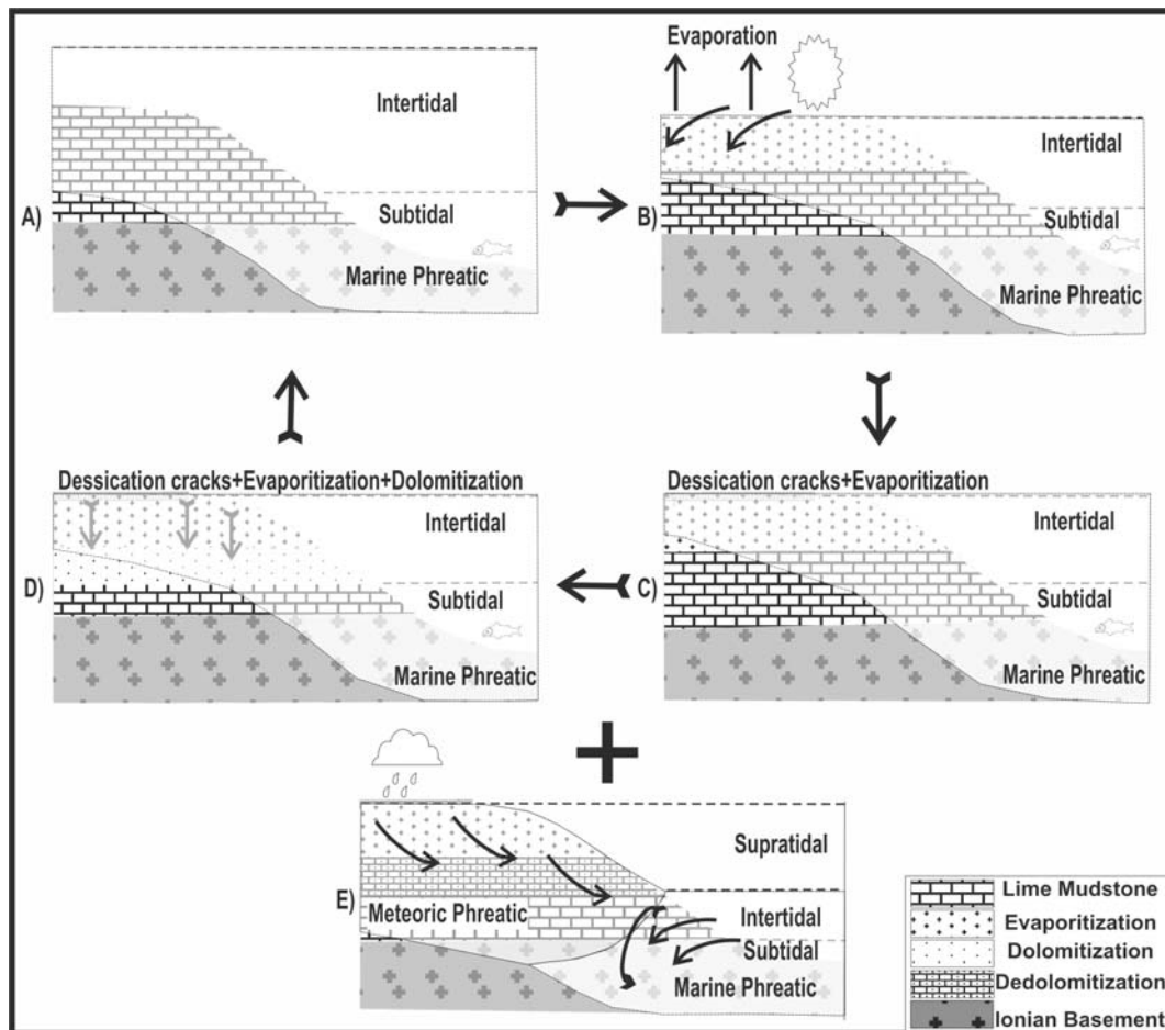
Figure 4. Sedimentation and diagenesis processes. See text for more details.
