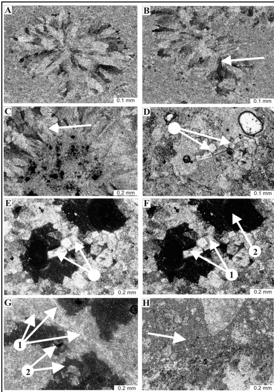
Figure 3. (A) Evaporitic rosette, cross polars, (B) Radiaxial or fibrous pore filling cement, cross polars, (C) Radiaxial cement, (D) Dolomitic rhombs, (E) Dolomitic rhombs, (F) 1: Dolomitic rhombs 2: Vugs, cross polars, (G) 1: Desiccation cracks 2: Vugs, (H) Red Brown cement showing diagenesis during subaerial exposure.
