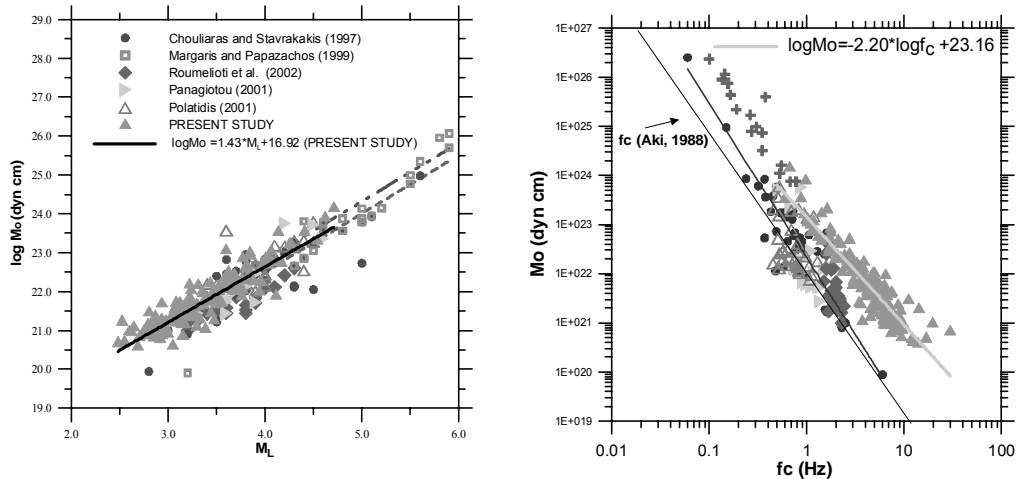
Figure 5. Left Part : Seismic moment, M_o , versus M_L : Comparison between the results derived in the present study and those from Chouliaras and Stavrakakis (1997), (solid circles), Margaris and Papazachos (1999), (open square), Panagiotou (2001), (solid triangle), Polatidis (2001), (open triangles) and Roumelioti et al. (2002), (solid diamond). Black and gray thin lines are equations proposed by Margaris and Papazachos (1999) and Roumelioti et al. (2002), respectively. The black thick line corresponds to equation (1) proposed in this study. Right Part : Seismic moment, M_o , variation versus corner frequency, f_c . The symbols have the same meaning as in the left part of the figure 1. Black and gray thin lines are relations proposed by Aki (1988) and Chouliaras and Stavrakakis (1997) respectively, while the gray thick line is proposed in the present study (equation 3).
