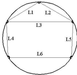
Figure 6. Drawing of a typical control section of Acheloos Diversion Tunnel. The 6 distances repeatedly measured with a convergence tape are marked L1 to L6.
