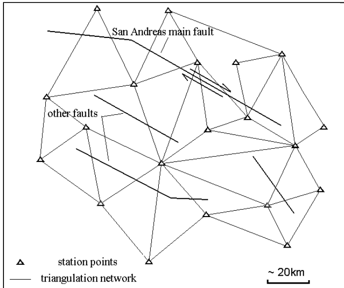
Figure 3. Map of a triangulation network at San Andreas Fault zone, California established for studying the strain tensor. Major faults are shown in black lines. Despite faulting, strain is assumed uniform, i.e. depending on the azimuth of the observation line only. After Savage (1983) simplified.
