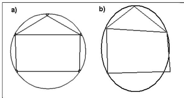
Figure 2. a) Observed line length changes across a tunnel section, using a tape, b) sketch of the deformed section (exaggerated): observations are not compatible with each other, and extended lines do not fit to an ellipse, mainly due to measurements errors.
