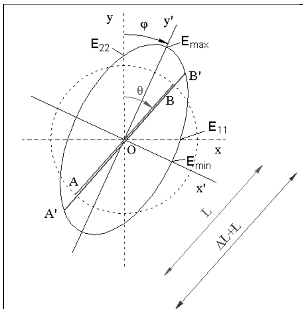
Figure 4. Geometric representation of our model, a circle (corresponding to a part of the earth's surface) deformed to an ellipse. All parameters for calculating the strain field based on the Frank's (1966) theory are shown.
