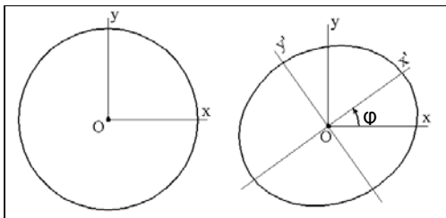
Figure 5. Due to strain, a circle of unit radius is transformed to an ellipse. Equations and techniques described above permit to calculate the length and orientation of the main axes of this ellipse.
