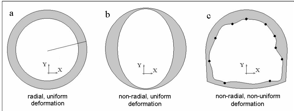
Figure 1. A sketch to show different types of strain field across tunnels (simplified from Kontogianni et al. 2004).
