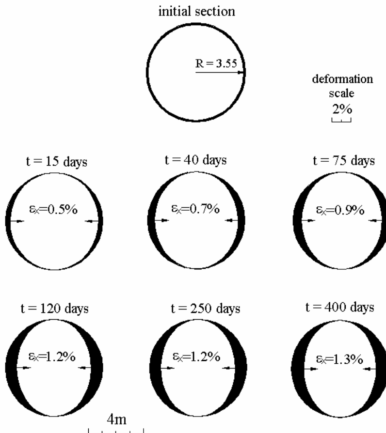
Figure 8. Progressive change of the section strain field along time. Horizontal strain ( \epsilon_x ) accumulates gradually to 1.3% (corresponding to maximum strain), whereas vertical strain remains 0.
