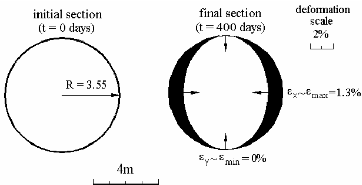
Figure 7. Schematic comparison of the initial and of the final (exaggerated) form of a representative section of Acheloos Diversion Tunnel (ch. 16+276m), 400 days after the excavation.
